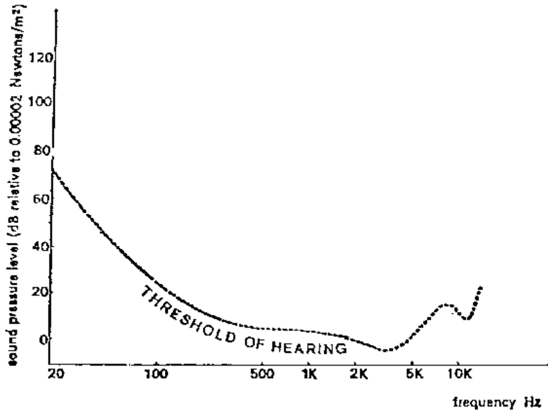
Figure 2-2. Average threshold of hearing. Source: Ref. 13, p. 12.
