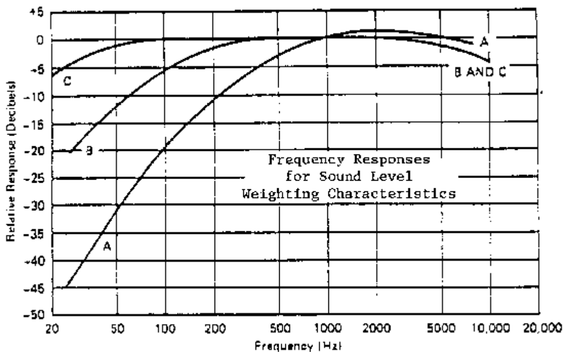
Figure 7-1 Frequency responses for sound level weighting characteristics.
