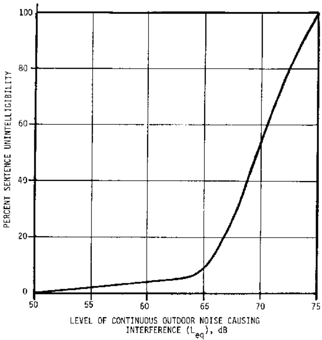
Figure 4-2 Criteria for outdoor speech interference (normal voice at 2 meters)
