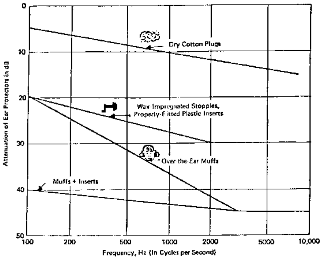
Figure 2-10 Sound attenuation characteristics of various types of ear protectors Source: Ref. 23
