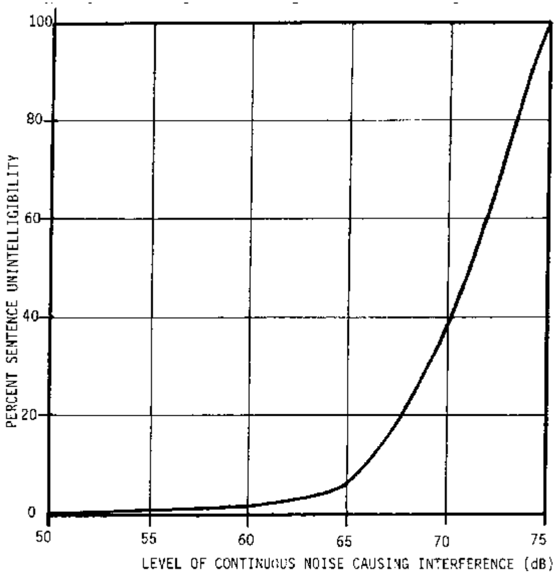
Figure 4-1 Criteria for indoor speech interference (relaxed conversation at greater than 1 meter separation, 45 dB background in the absence of interfering noise) Source: Ref. 5.
