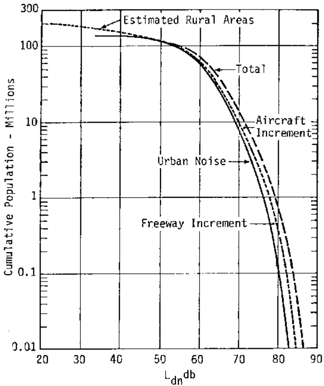
Figure 1-2 Residential noise environment of the national population as a function of exterior day-night average sound level. Source: Ref 5
